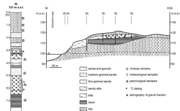
Fig. 2. Geological situation of mollusc-bearing deposits at Wildno in Dobrzyń Lakeland (after Dzierżek, Szymanek 2013, modified).
